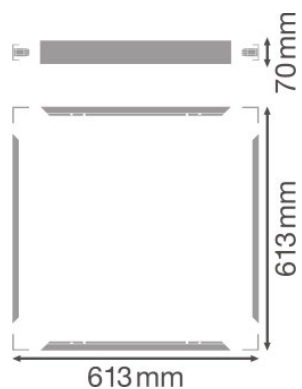
PANEL 600 SURFACE MOUNT KIT H70 VAL
