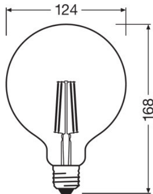
SMART+ Filament WiFi Classic Globe 60 5,5W E27
